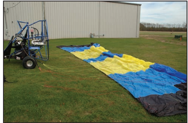
Figure 7-1. The inverted method of laying out the wing.
